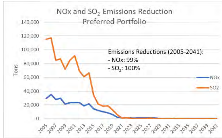
Figure 59: I&M Preferred Portfolio SO 2 and NO x Emissions Reductions
